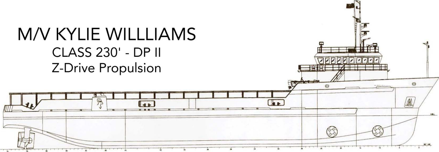
OUTBOARD PROFILE
